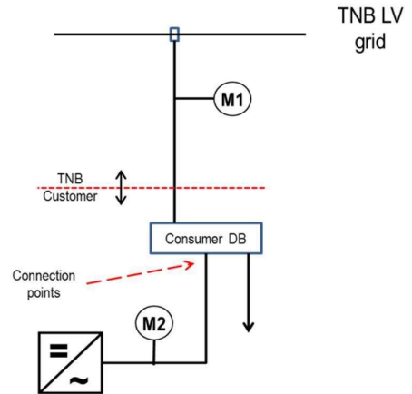
Fig. 5.3: Type A connection
