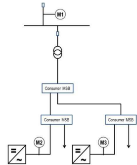
Fig. 9.1: Location of Energy Meters
