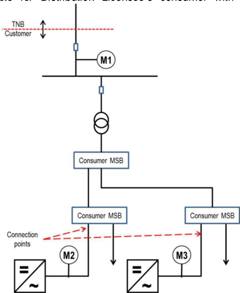
Fig. 5.4: Type B connection
